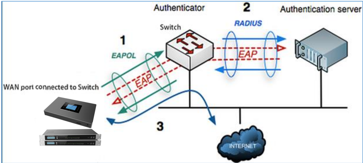
Figure 22: UCM630X Using 802.1X as Client
