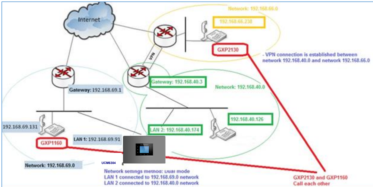
Figure 24: UCM6304 Static Route Sample
