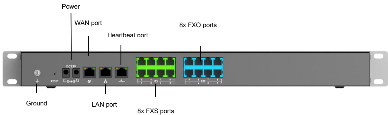
Figure 9: UCM6308 Back View
