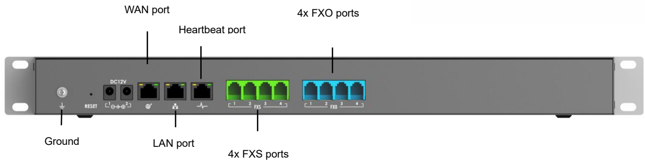
Figure 7: UCM6304 Back View
