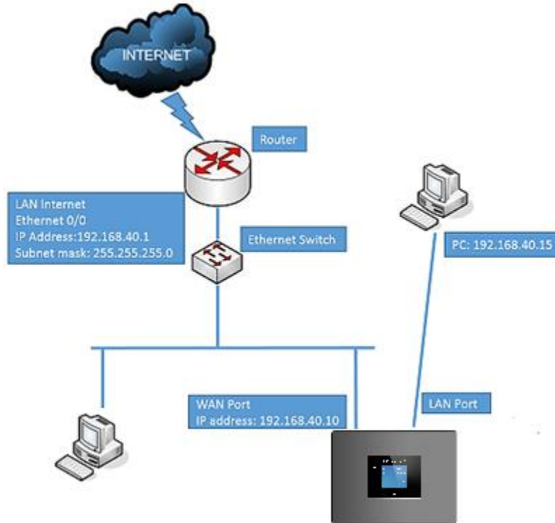
Figure 20: UCM6302 Network Interface Method: Switch
