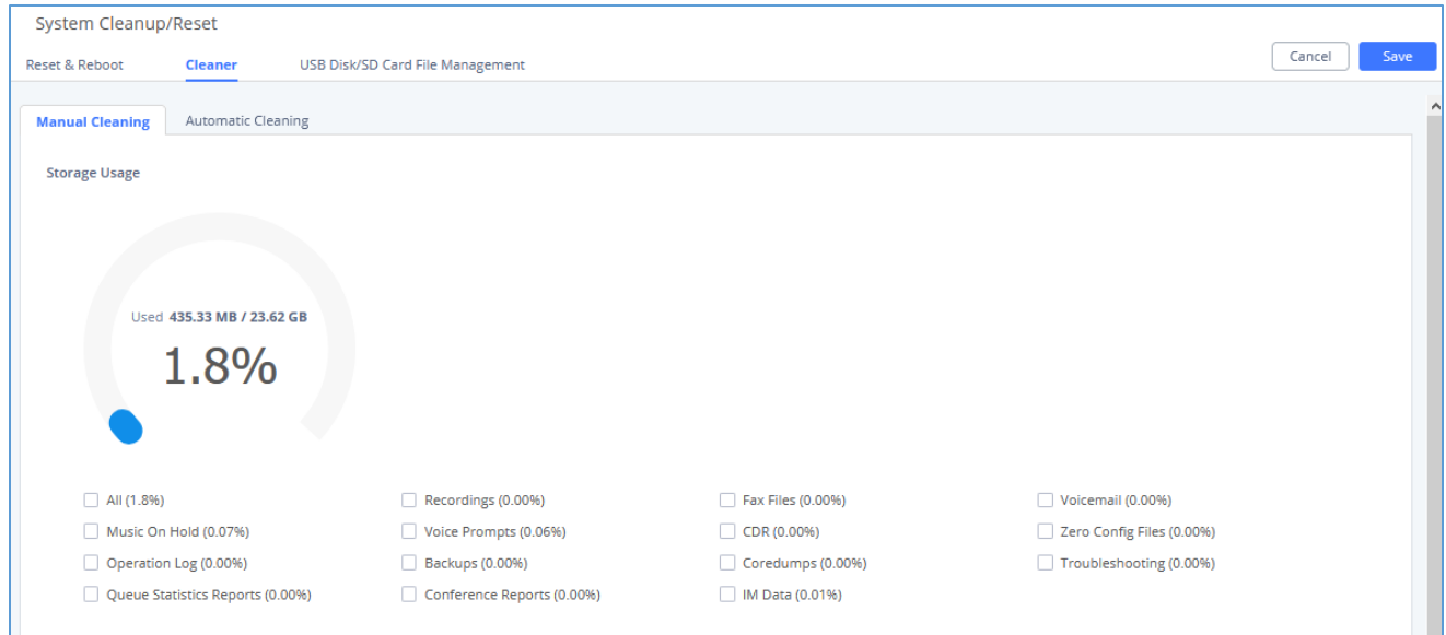
Figure 363: Manual Cleaning
