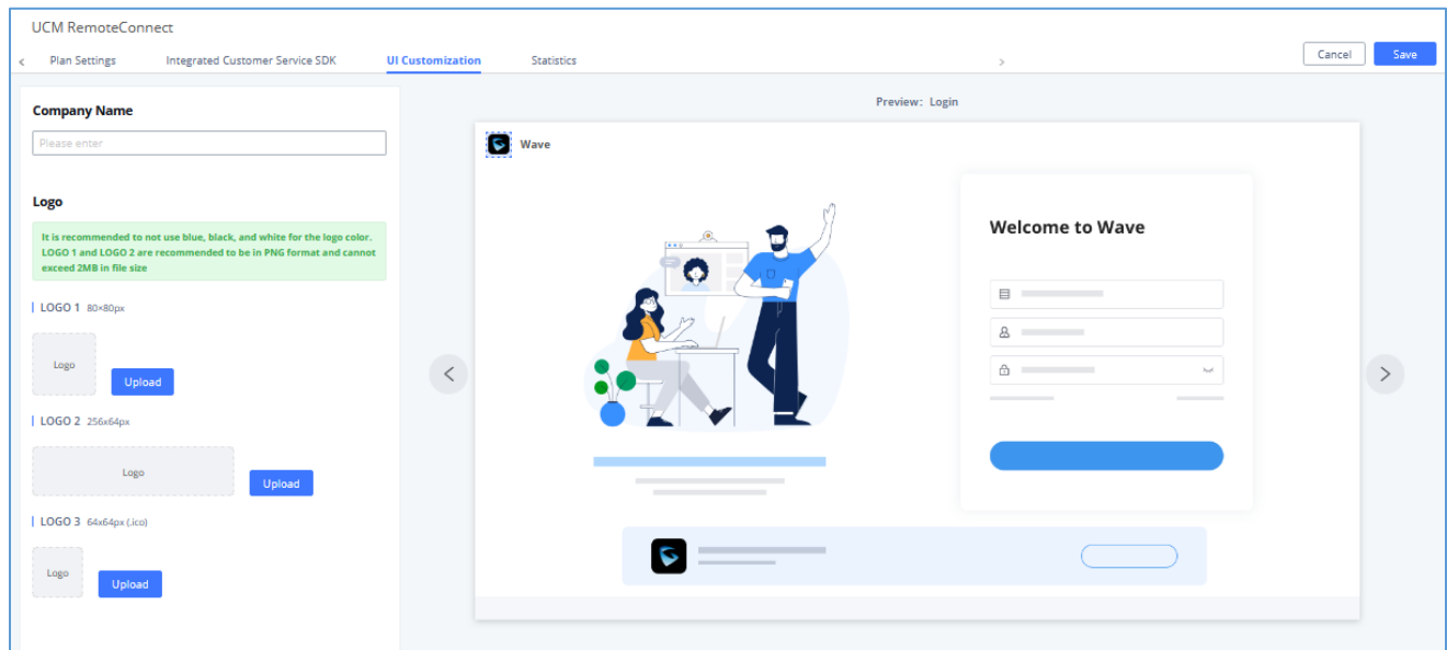
Figure 264: UI Customization
