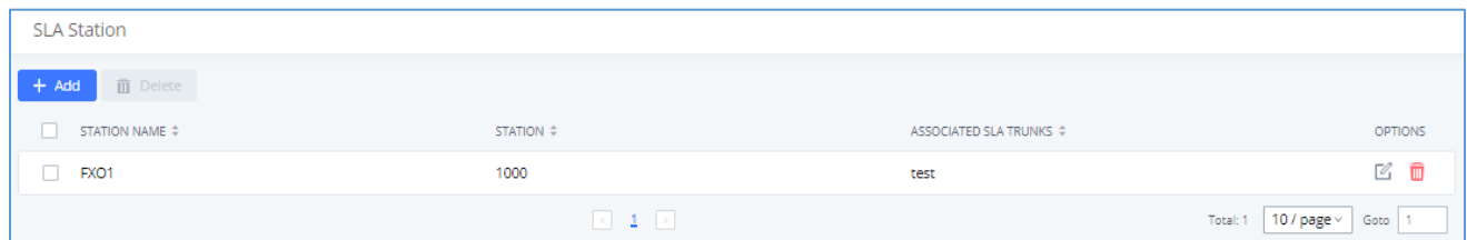
Figure 111: SLA Station
