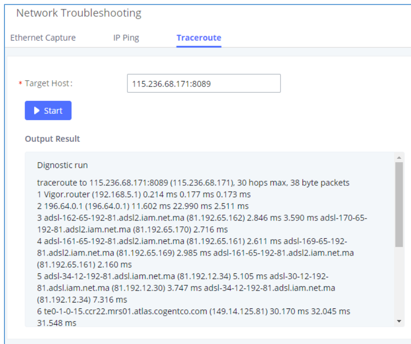
Figure 370: Traceroute
