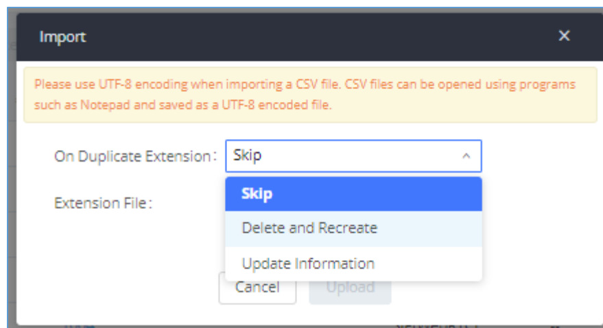
Figure 91: Import Extensions
