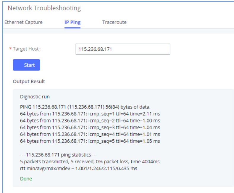
Figure 369: Ping
