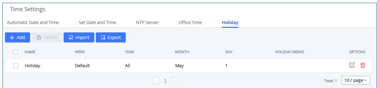
Figure 56: Settings→Time Settings→Holiday
