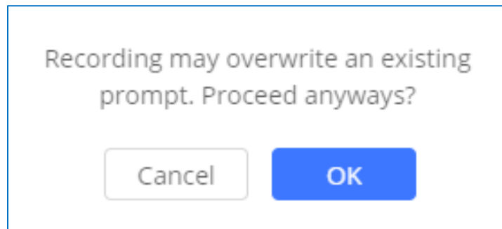
Figure 209: Information Prompt
