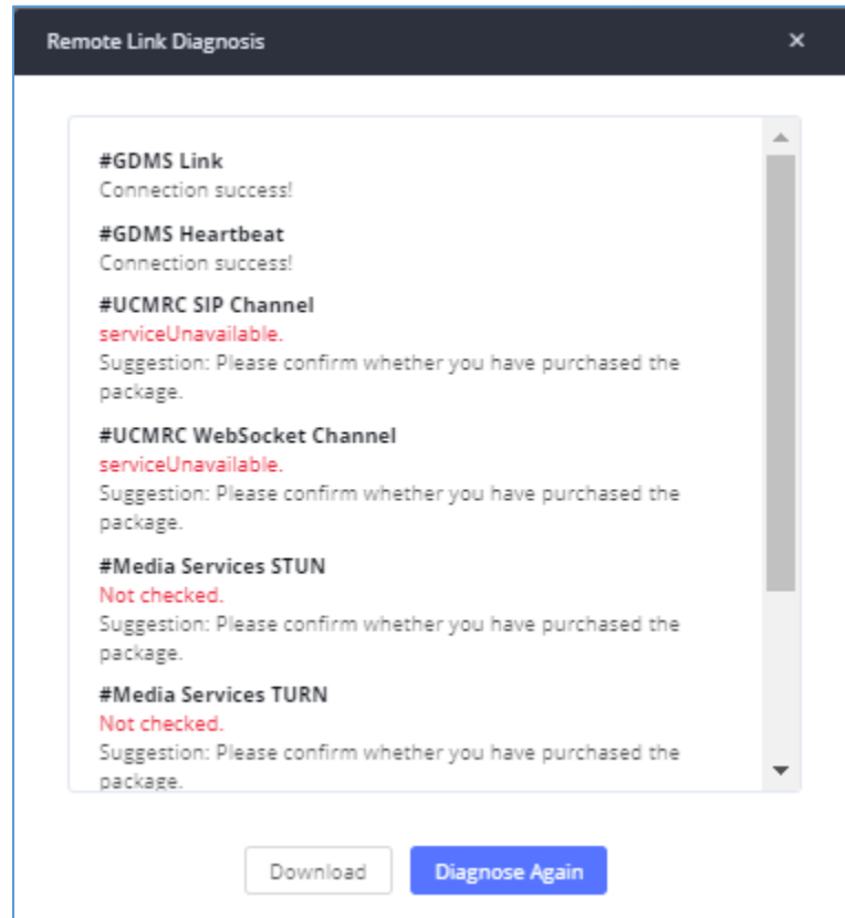
Figure 259: Remote Diagnosis
