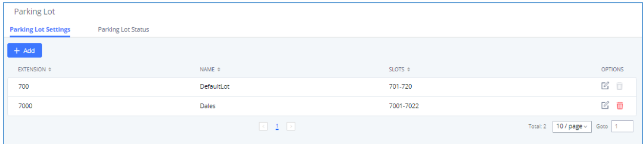
Figure 232: Parking Lot
