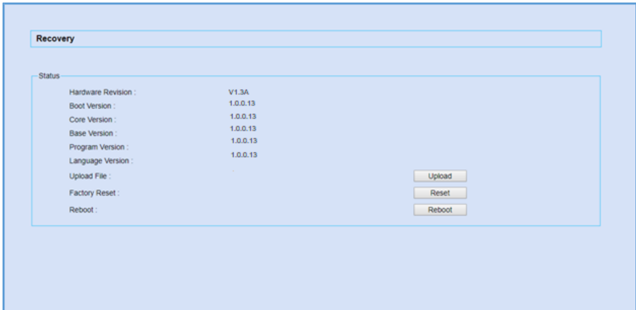
Figure 367: Recovery Mode
