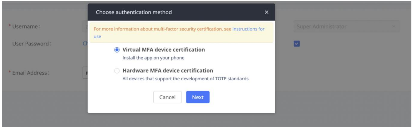
Figure 334: MFA Settings
