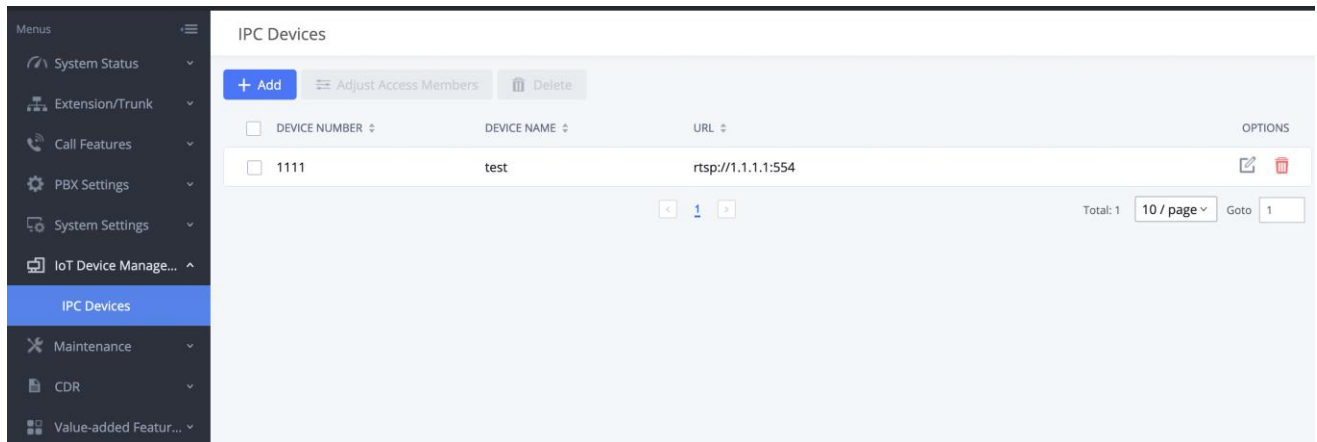
Figure 256: IPC Devices
