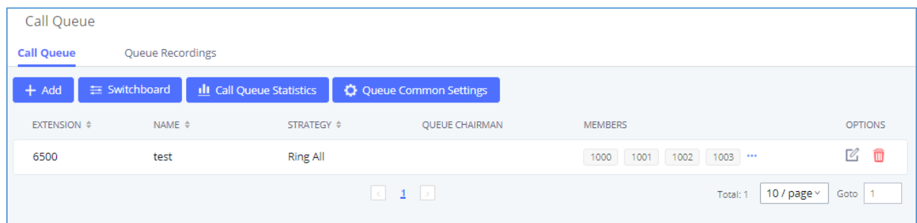
Figure 191: Call Queue
