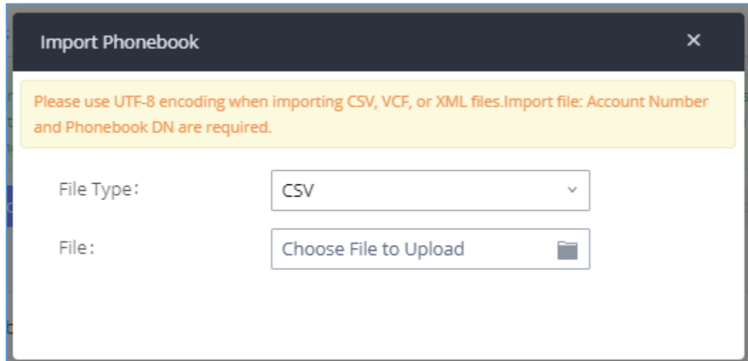
Figure 43: Import Phonebook
