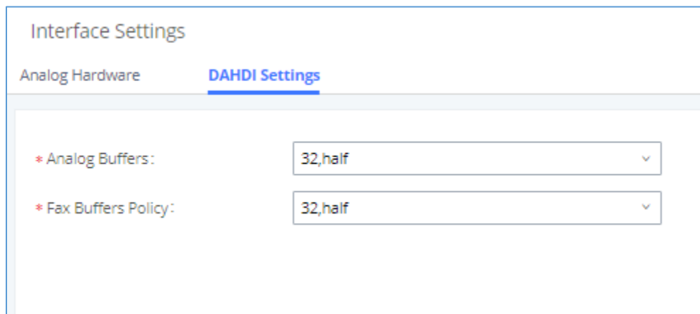
Figure 255: DAHDI Settings
