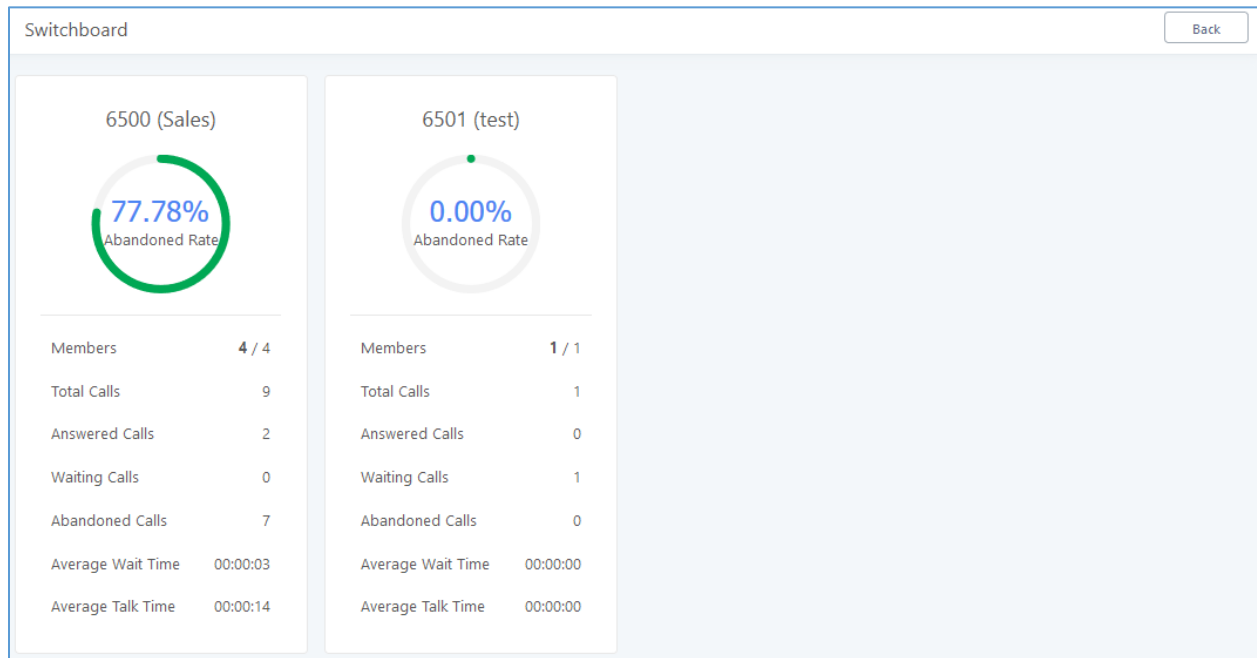
Figure 199: Switchboard Summary
