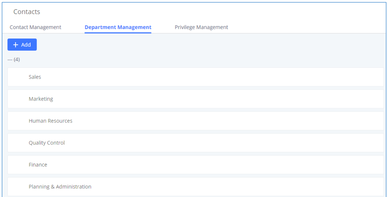
Figure 343: Department Management
