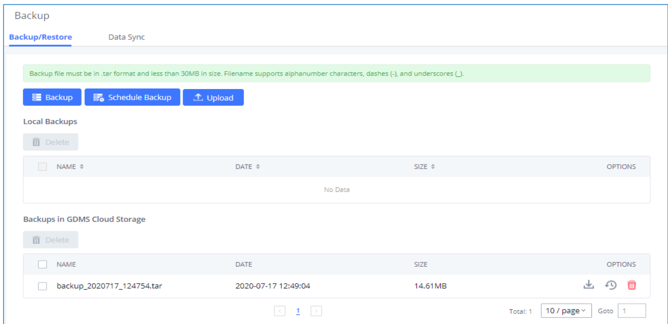
Figure 358: Backup / Restore
