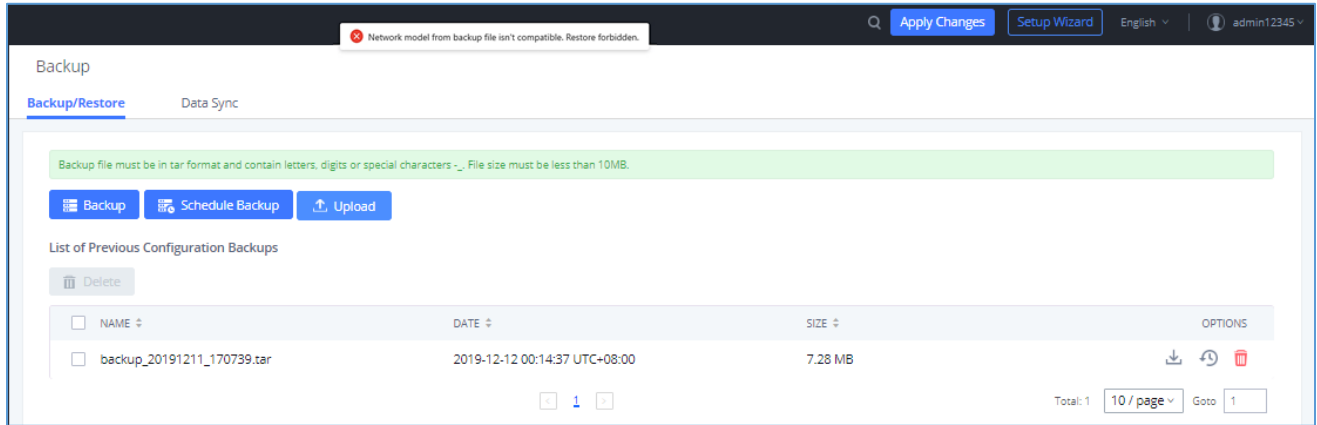
Figure 357: Restore Warning
