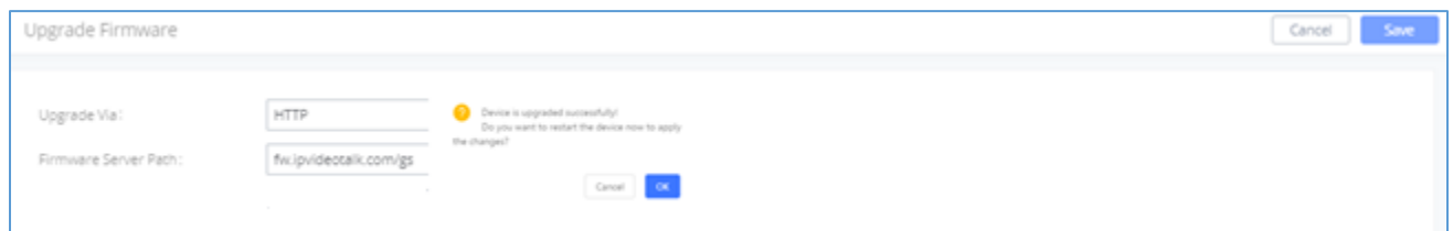
Figure 355: Reboot UCM630X
