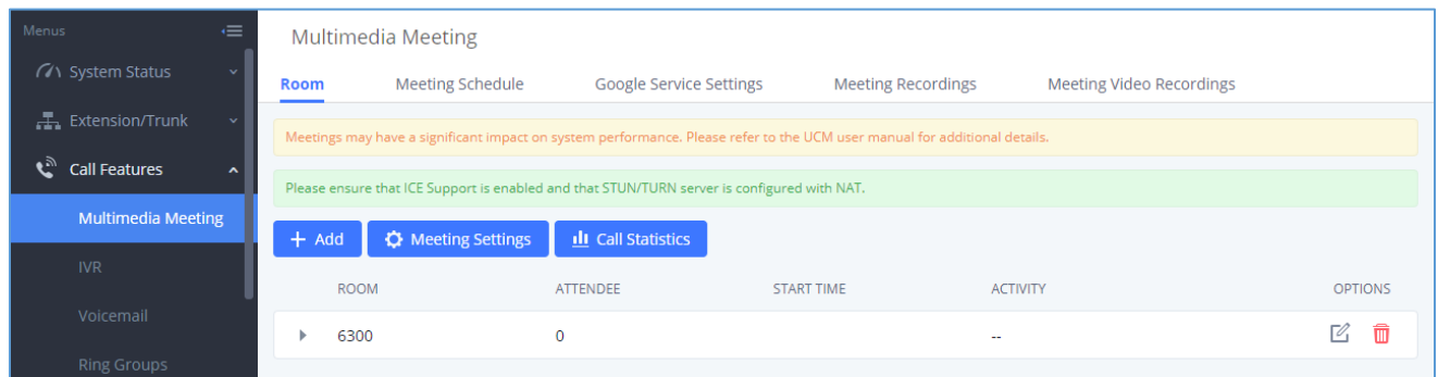
Figure 148: Multimedia Meeting
