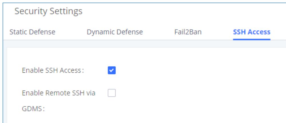
Figure 36: SSH Access
