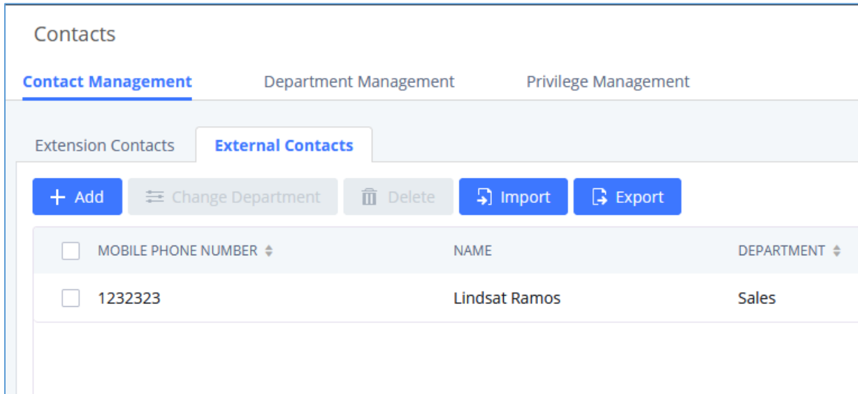
Figure 341: External Contacts
