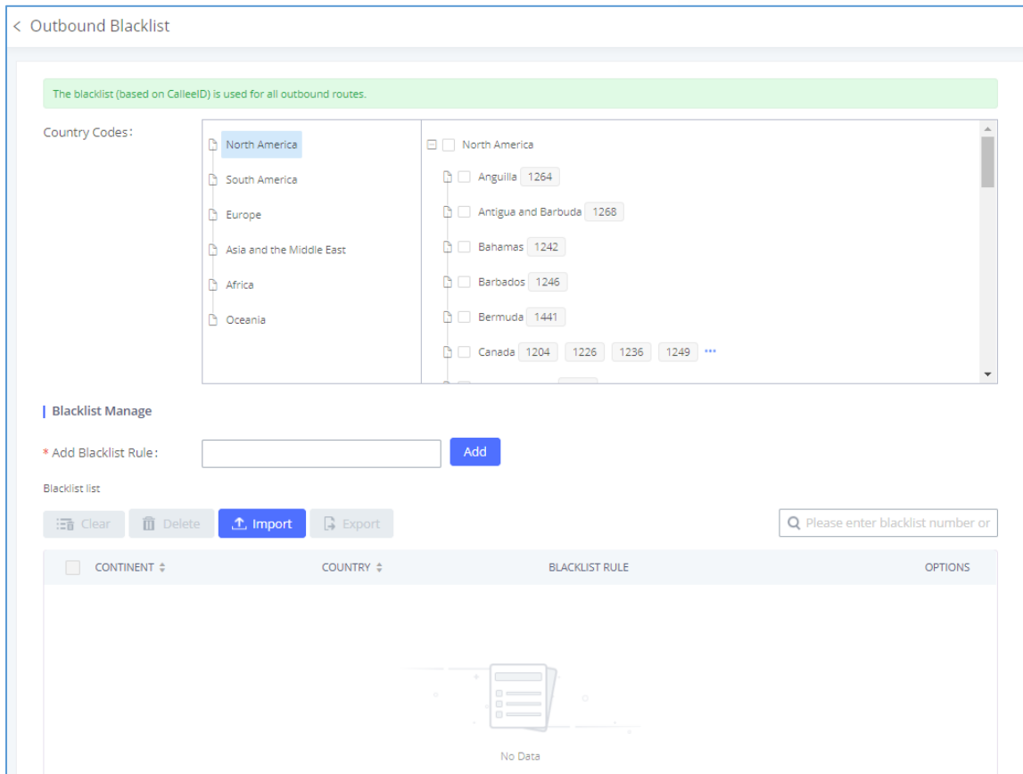
Figure 118: Country Codes
