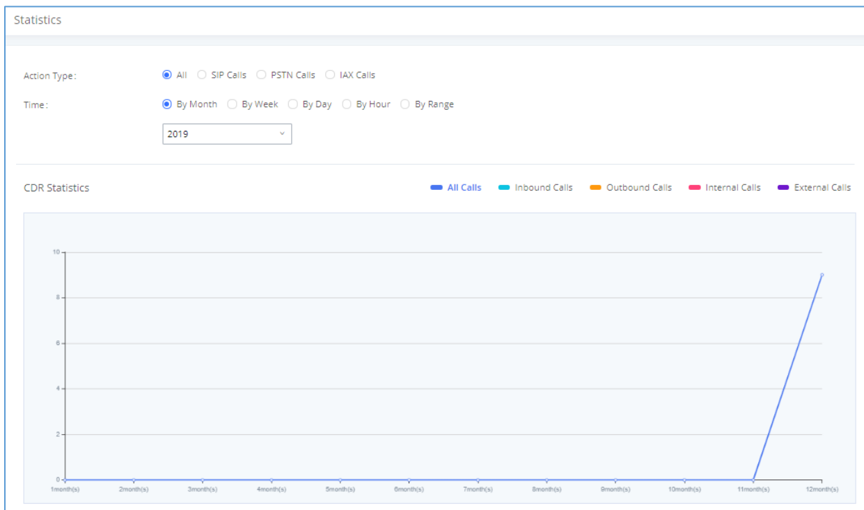
Figure 326: CDR Statistics
