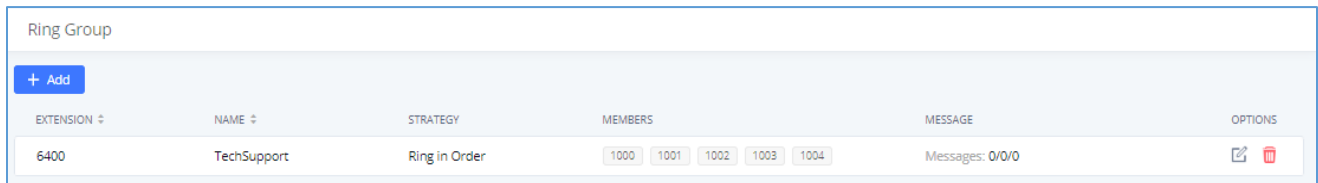
Figure 177: Ring Group
