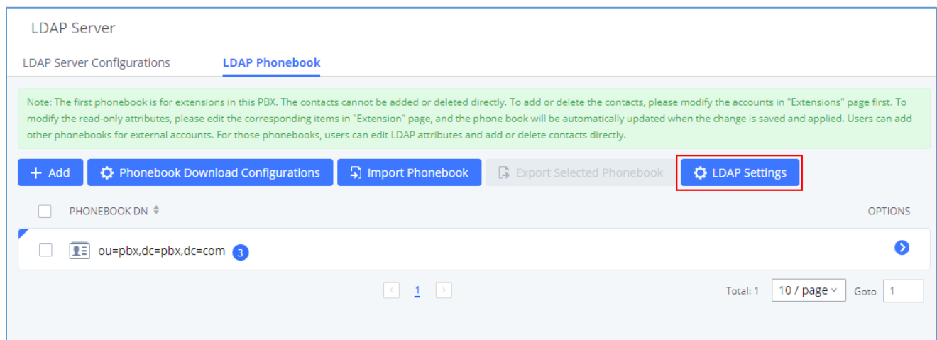
Figure 47: LDAP Settings
