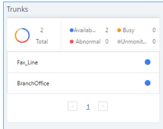
Figure 300: Trunk Status
