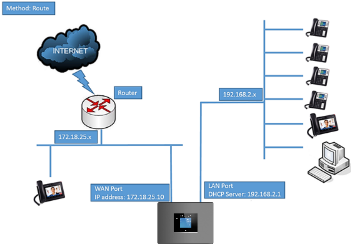
Figure 19: UCM6302 Network Interface Method: Route
