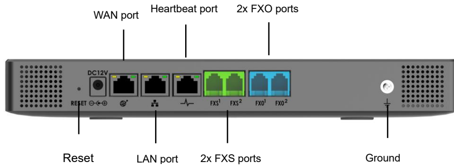
Figure 4: UCM6302 Back View
