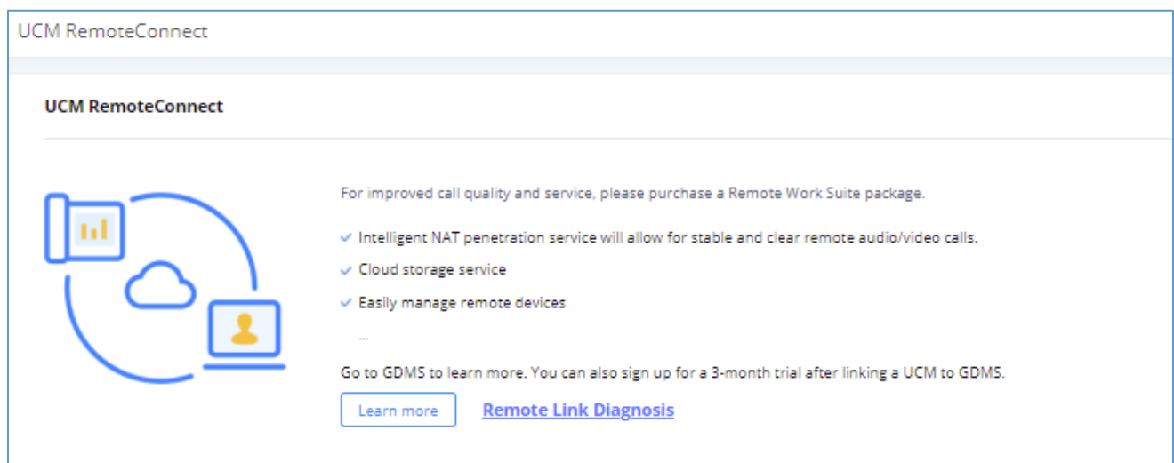
Figure 258: RemoteConnect
