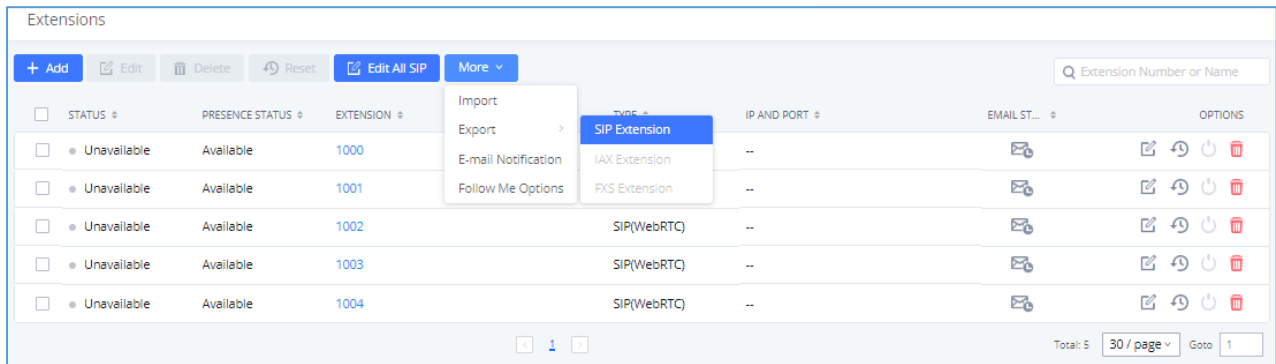
Figure 90: Export Extensions
