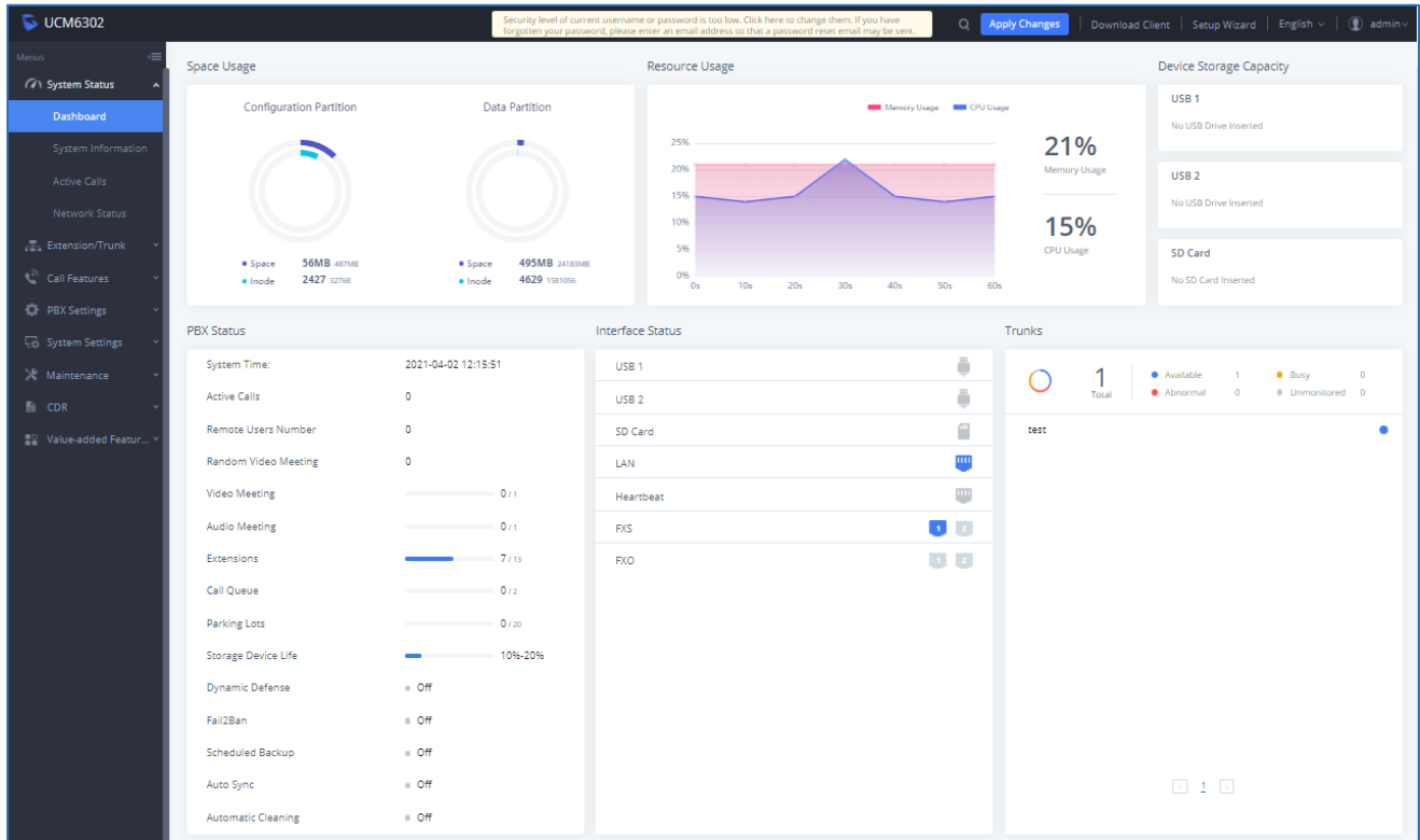
Figure 299: Status→PBX Status
