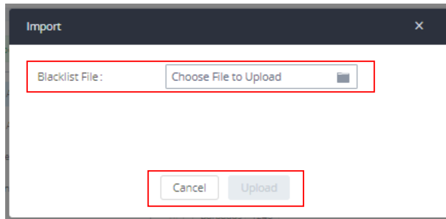
Figure 119: Blacklist Import/Export
