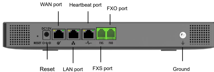
Figure 2: UCM6301 Back View
