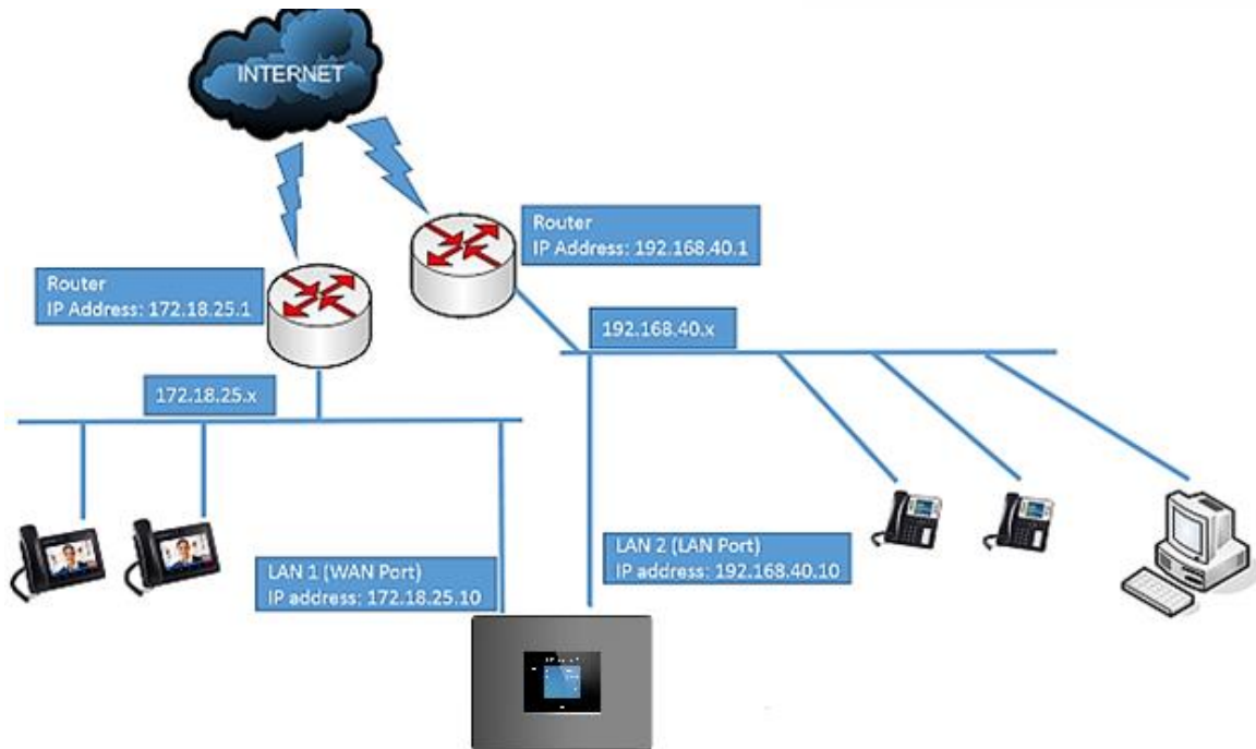
Figure 21: UCM6302 Network Interface Method: Dual
