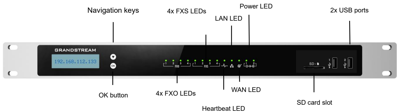
Figure 6: UCM6304 Front View
